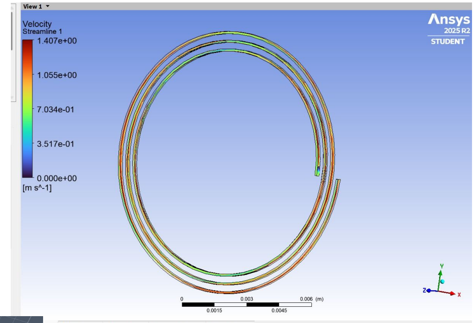
Fig. Simulated Spiral Microchannel
