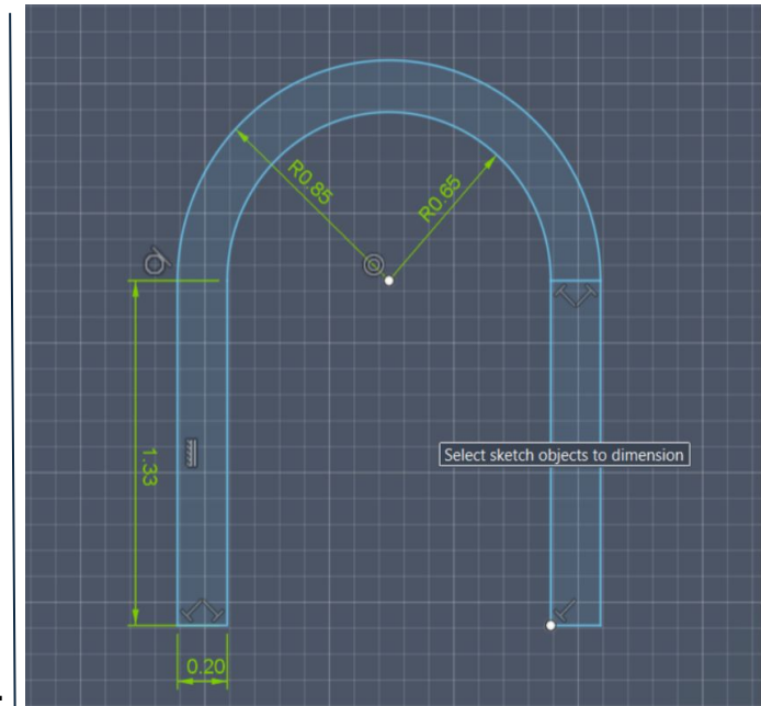
Fig. Schematic diagram of U-Bent Microchannel
