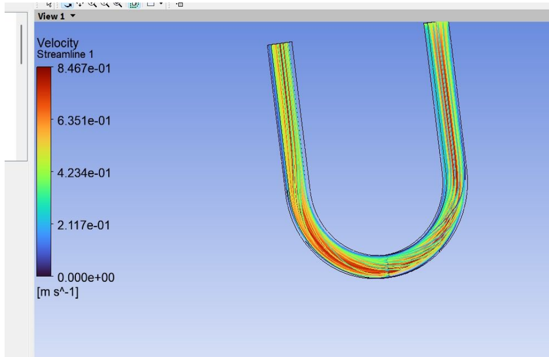
Fig. Simulated U-Bent Microchannel
