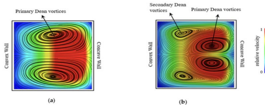
Fig. Rectangular cross section
