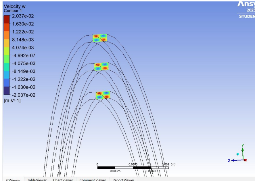
Fig. Dean Vortices
