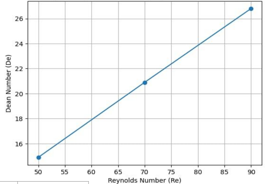
Graph of Reynolds Number (Re) vs Dean Number (De)
